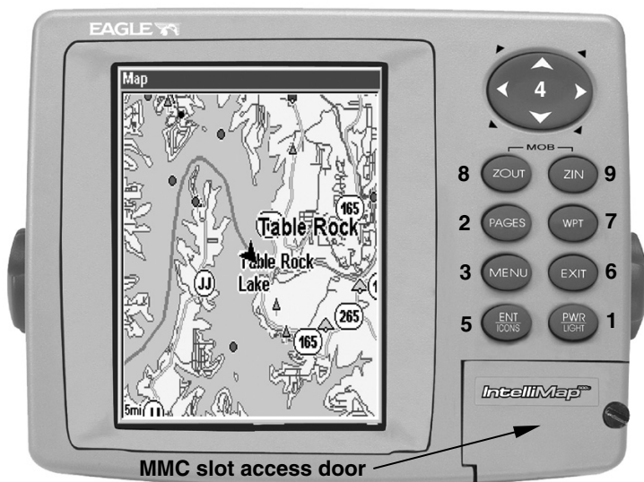
IntelliMap 502C GPS unit, front view, showing Map Page, keyboard and access door for the MMC slot.
